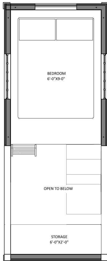
Loft floor plan
