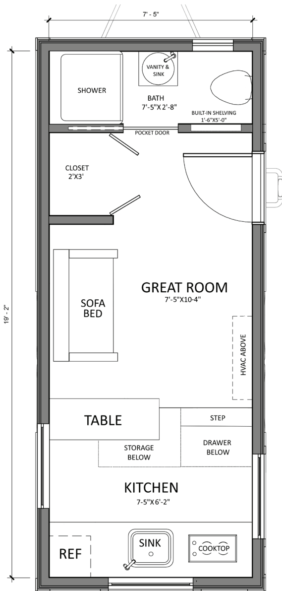
Floor plan
